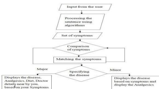
Figure 3: Data Flow Diagram
