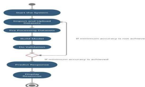
Figure 8 State/Activity Diagram
