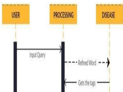
Figure 7 Interaction Diagram
