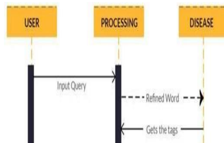
Figure 5 Sequence Diagram
